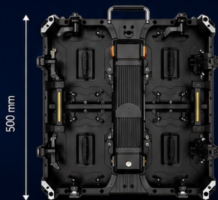
Rear view
